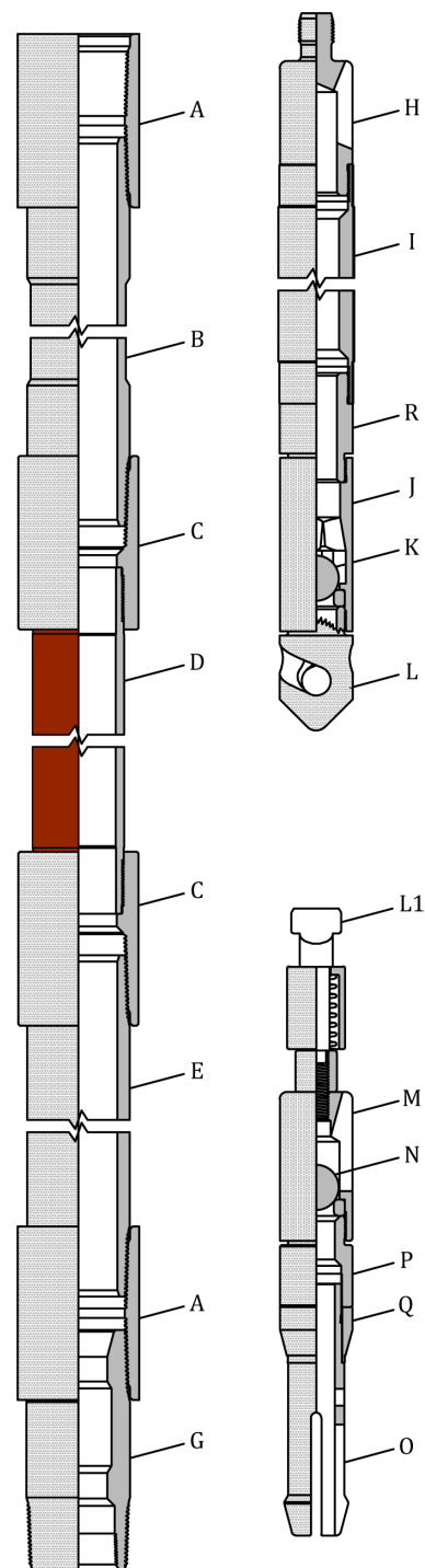
Stationary Assembly
