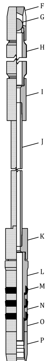
Stationary Assembly
