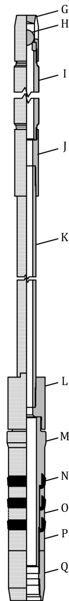
Stationary Assembly
